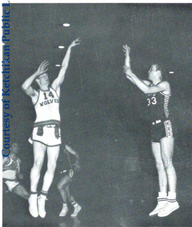
Seierup scores
